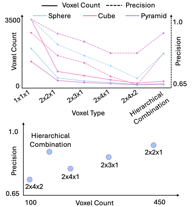
Figure 16: Evaluating voxel pattern efficiency— hierarchical combination outperforms any single voxel type by breaking the linear trade-off between voxel size and precision. (Top: Voxel count and precision decrease linearly with increasing voxel size when voxelizing meter-scale meshes. Bottom: Precision as a function of voxel count, highlighting the benefits of the hierarchical combination.)
